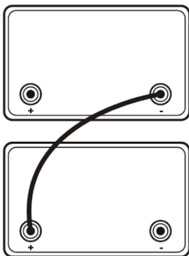
Series Connection
